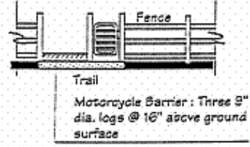
B: Elevation -- OHV Barrier
