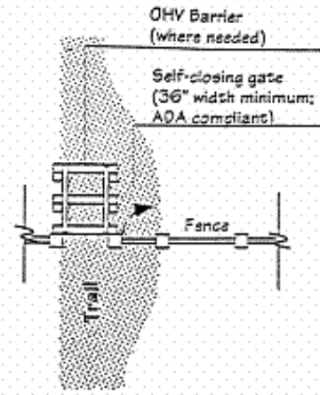
B: Plan -- OHV Barrier
