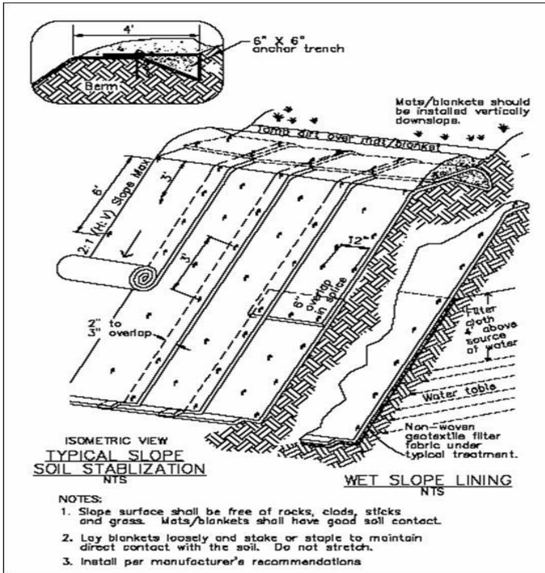
FIGURE EC-17-1 TYPICAL INSTALLATION DETAIL
