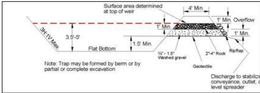
FIGURE SC-14-1 CROSS-SECTION OF SEDIMENT TRAP
