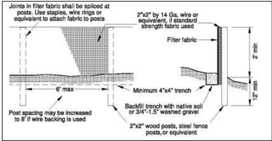
FIGURE EC-7-1 SILT FENCE
